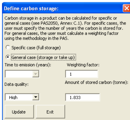
Figure 20 Carbon storage
